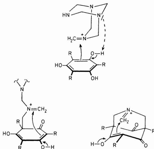
Scheme 1. Postulated intermediates.
